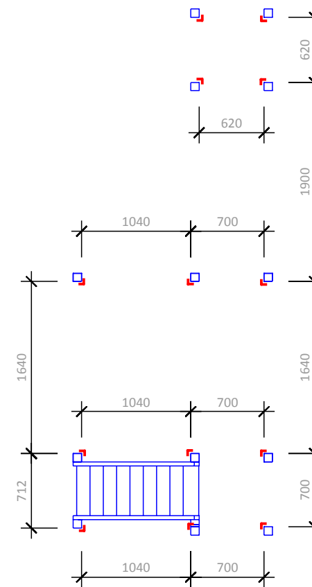
Fundamentplan ■ = 13 x Winkelanker
